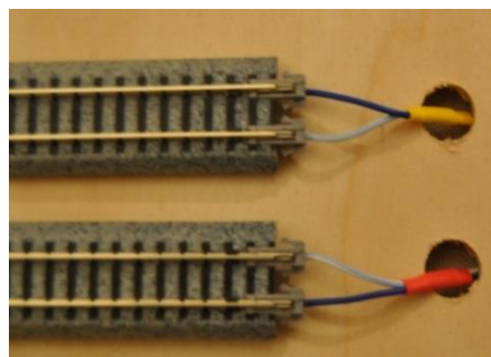
Tracks must be wired blue-white-white-blue
